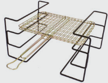
122/7 - Grid Stand Multilevel Material: 8 mm Mild Steel Size: 300 mm (h)
